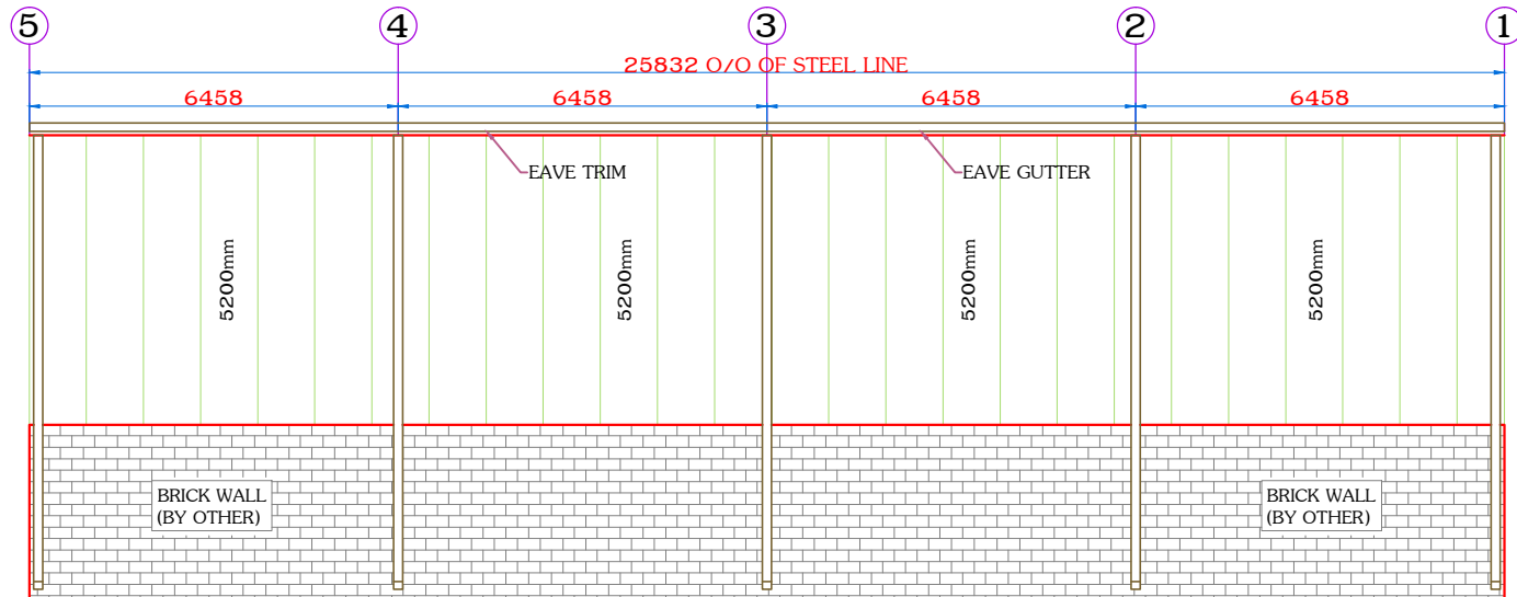
SIDE WALL SHEETING @ GRID-A
