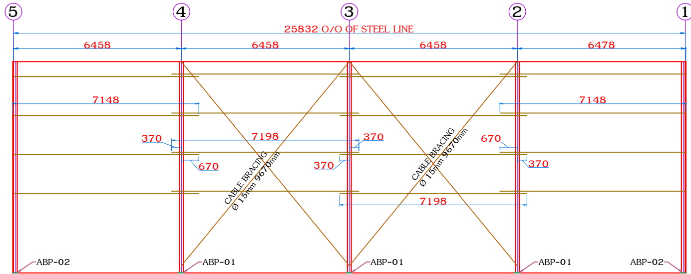
SIDE WALL FRAMING @ GRID-A
